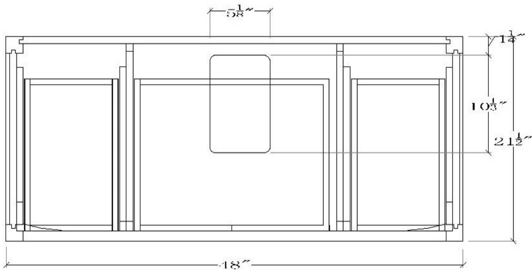
TOP VIEW
